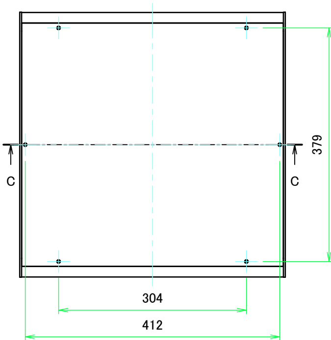
A view
